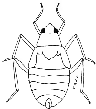
Fig. 358. Belostoma flumineum Soy, 5th instar.
